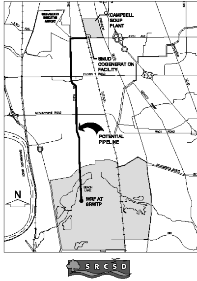
FIG. 1 VICINITY MAP POTENTIAL RECYCLED WATER SERVICE FOR CAMPBELL SOUP PLANT AND SMUD COGENERATION FACILITY
